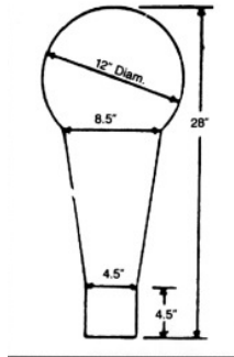
Fig. 3 - Speed Target.
